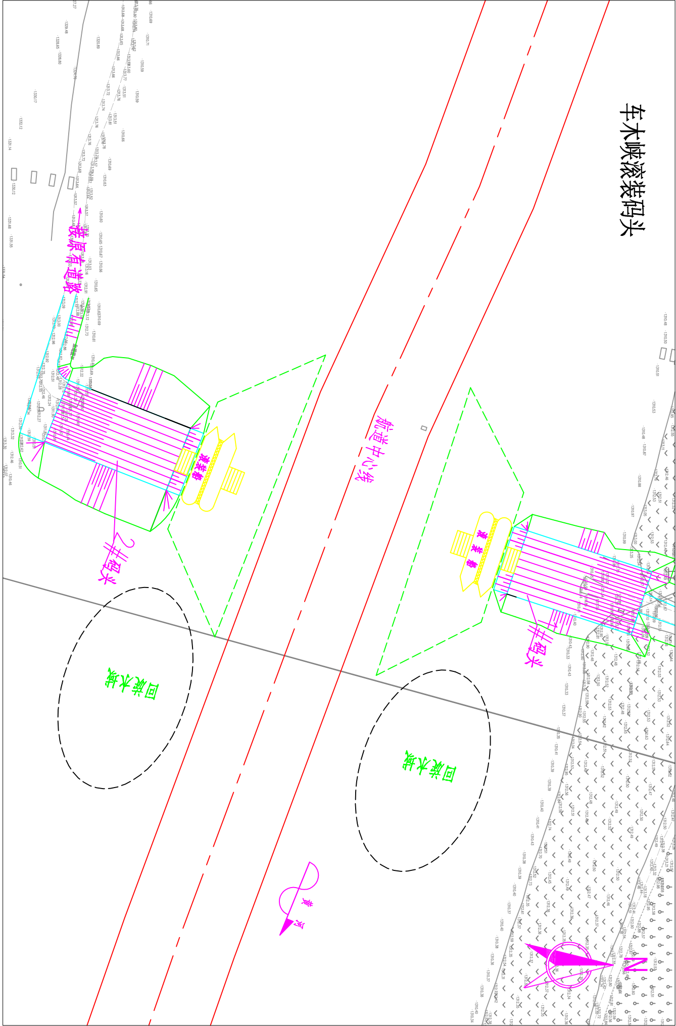
附图四 码头平面布置图(1/3)
